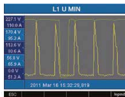
Fig.: Graphical event display (voltage drop)
